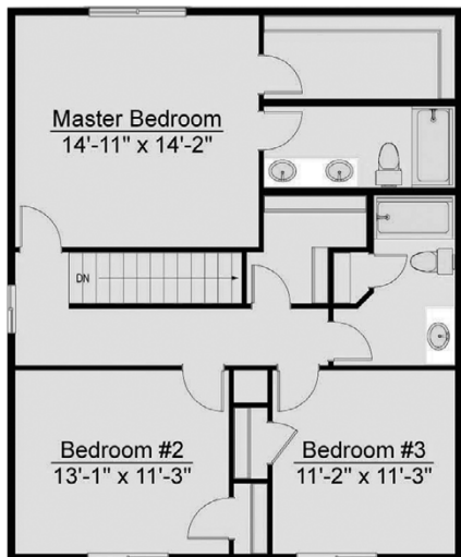
Upper Floor
